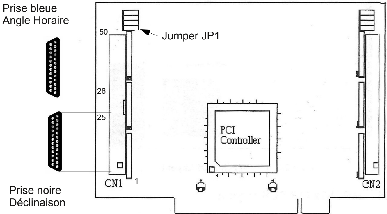
Figure 2-1: PCI-7248/7224 PCB Layout
